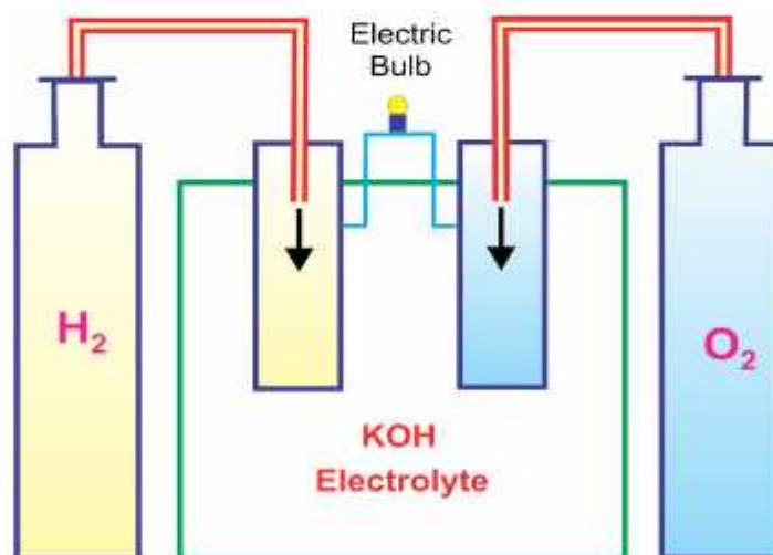
Fig. 14.2 Working of a Fuel cell
