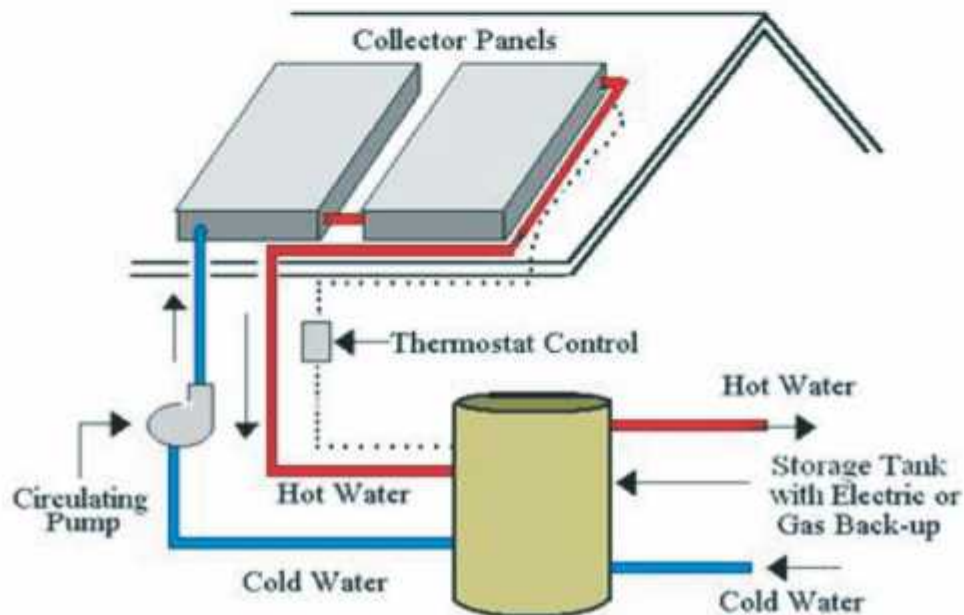
Fig. 13.2. Active Solar hot water heating system
