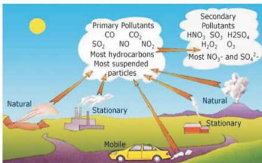
Fig. 7.1 Air Pollution
