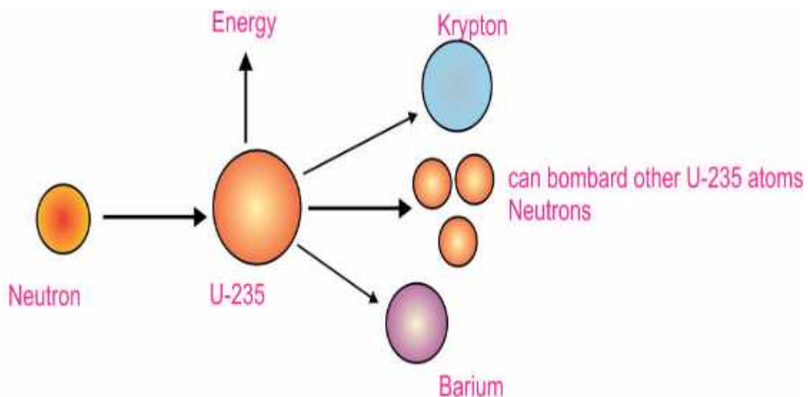
Fig 13.6 Nuclear Fission
