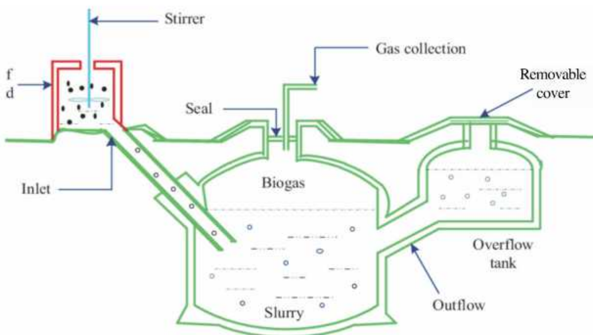
Fig 13.1 Biogas Plant
