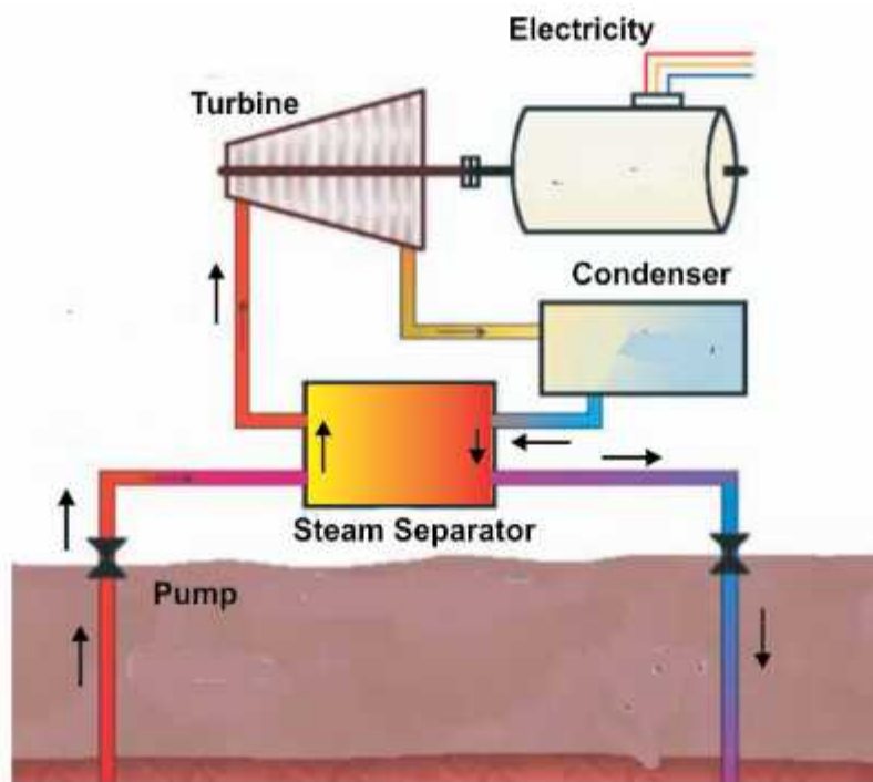
Fig. 13.5 Geothermal Power Plant
