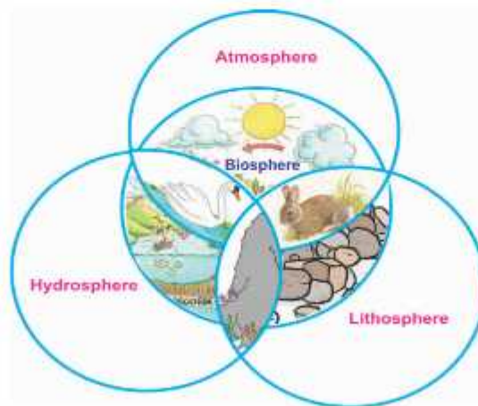
Fig 1.1 Biosphere
